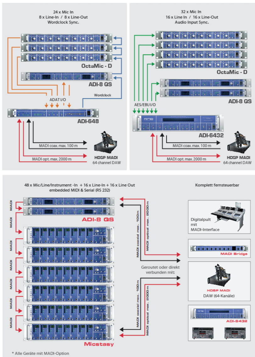
Grafik 3.6: MADI Front End Design 76
